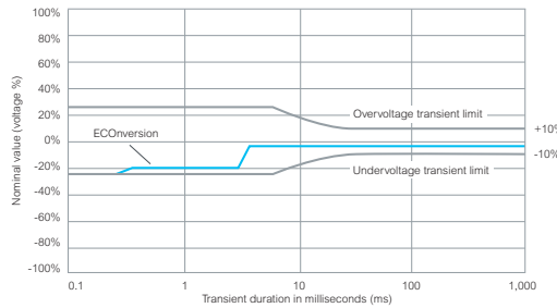
Galaxy VX ECONversion meets Class 1 of IEC 62040-3: Zero-break transfer during power outage
